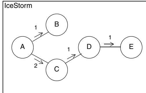
Figure 43.6. Initial graph.
