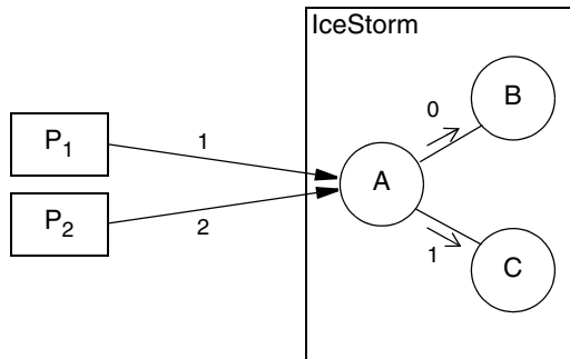
Figure 43.5. Cost semantics.
