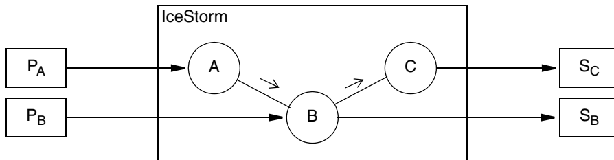
Figure 43.4. Message propagation.
