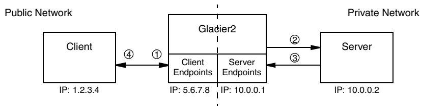
Figure 41.6. A callback via Glacier2.
