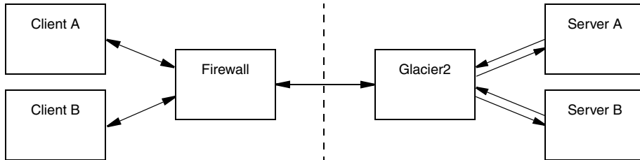
Figure 41.4. Multiple clients and servers with callbacks using Glacier.
