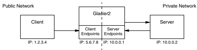
Figure 41.5. Glacier2’s client and server endpoints.
