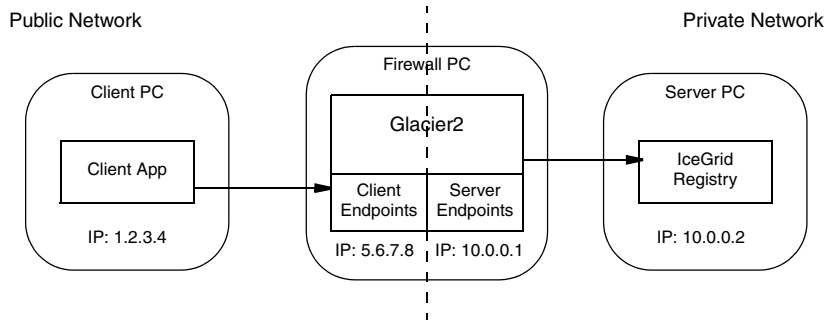
Figure 37.6. Using IceGrid via a Glacier2 router.
