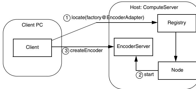
Figure 37.4. Architecture for initial ripper application.
