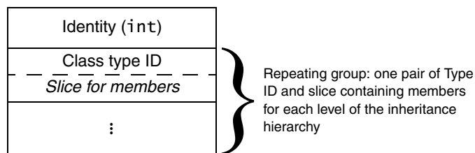
Figure 34.2. Marshaling format for classes.
