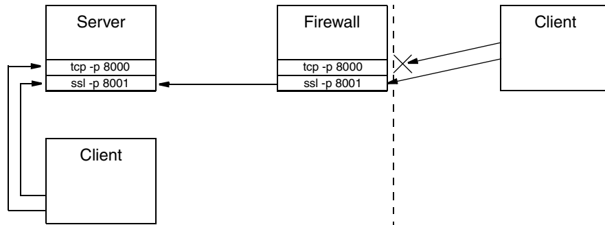
Figure 40.1. An application of multiple protocol endpoints.
