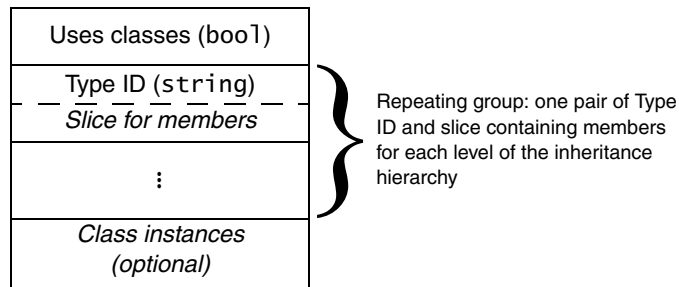
Figure 34.1. Marshaling format for exceptions.
