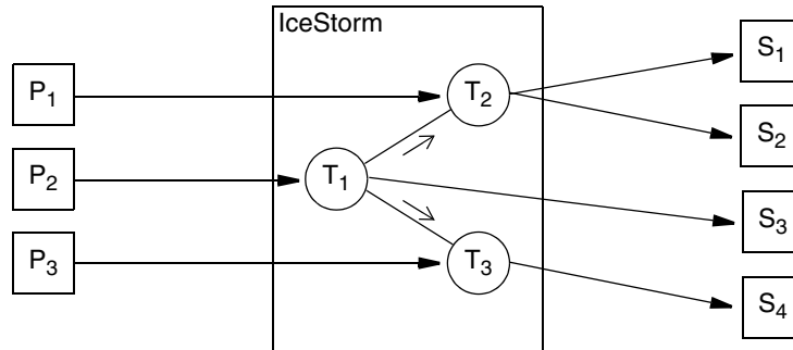
Figure 43.3. Topic federation.
