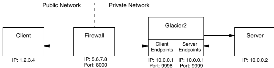
Figure 41.7. Using Glacier2 with a network firewall.
