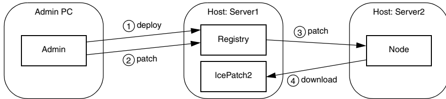
Figure 37.5. Overview of application distribution.
