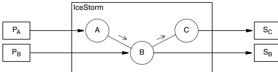
Figure 42.4. Message propagation.
