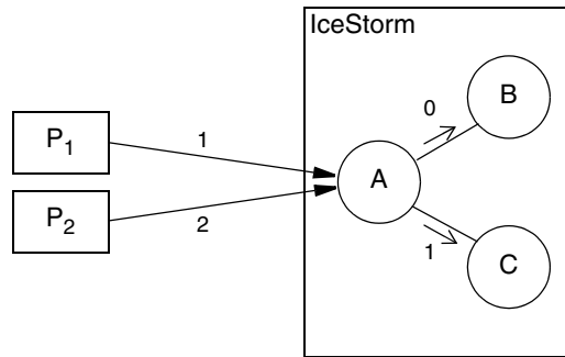
Figure 42.5. Cost semantics.
